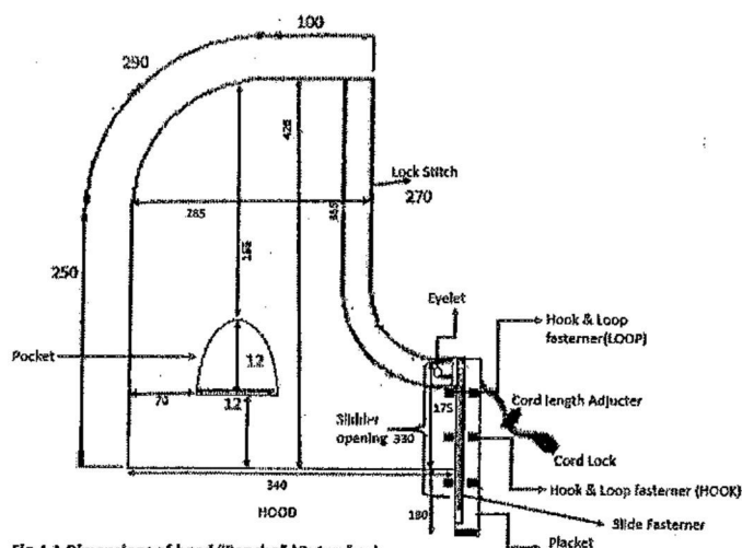
Fig-4 A Dimensions of hood "Poncho" {Outerview} (All the dimensions are in mm)
