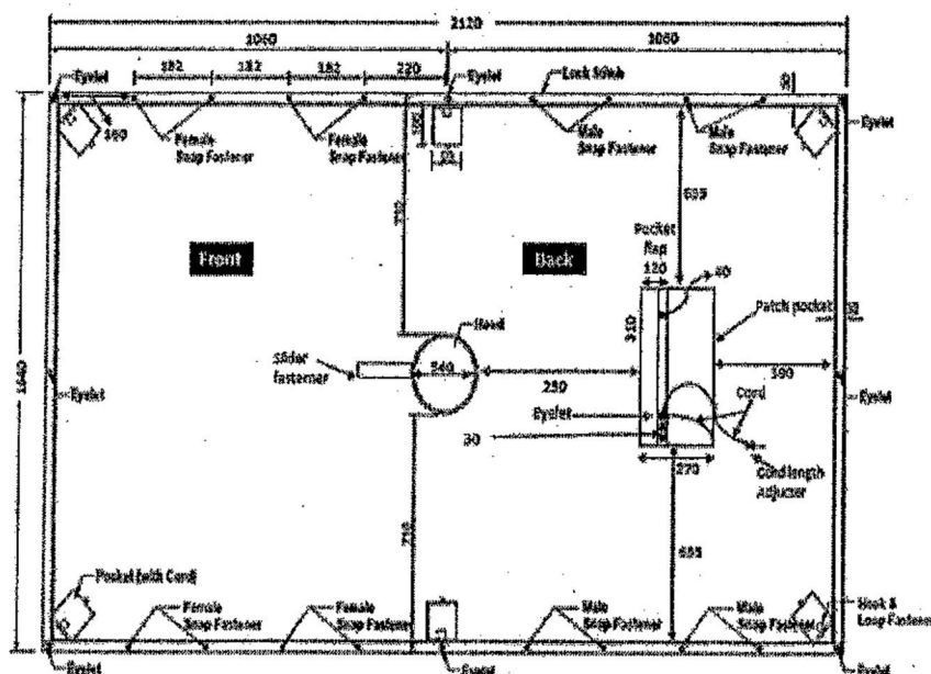
Fig: 3B Poncho (Inner view)
