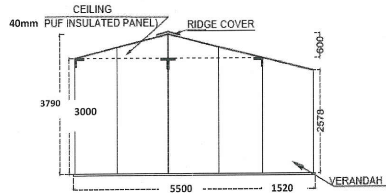
SIDE VIEW
