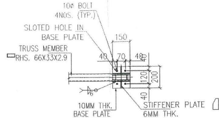
(TYP.) P3 & P4 BASE PLATE DETAIL (SLOTTED HOLES)
