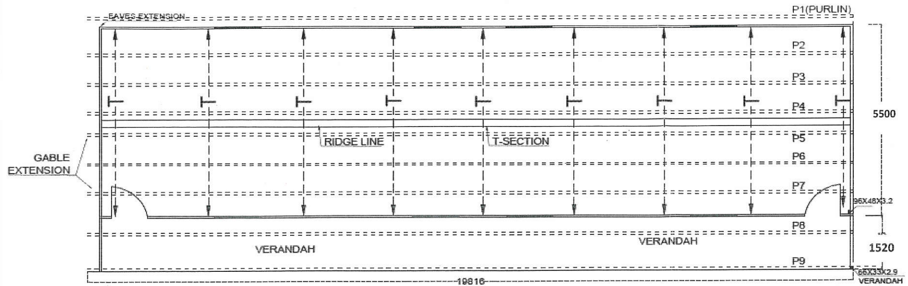
SPAN WITH VERANDAH
