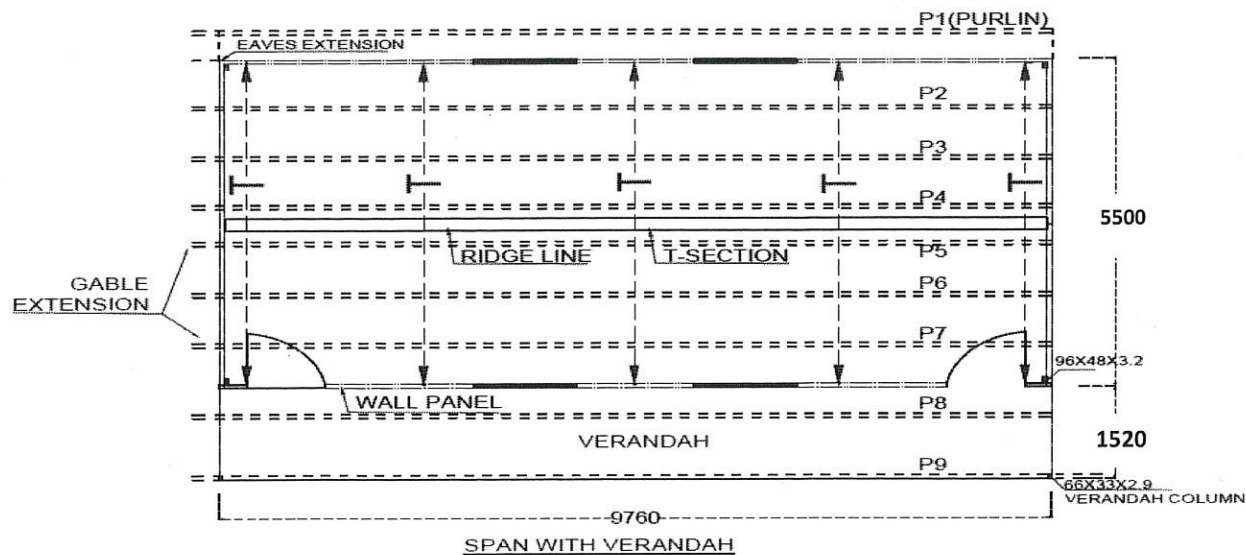
SPAN WITH VERANDAH
