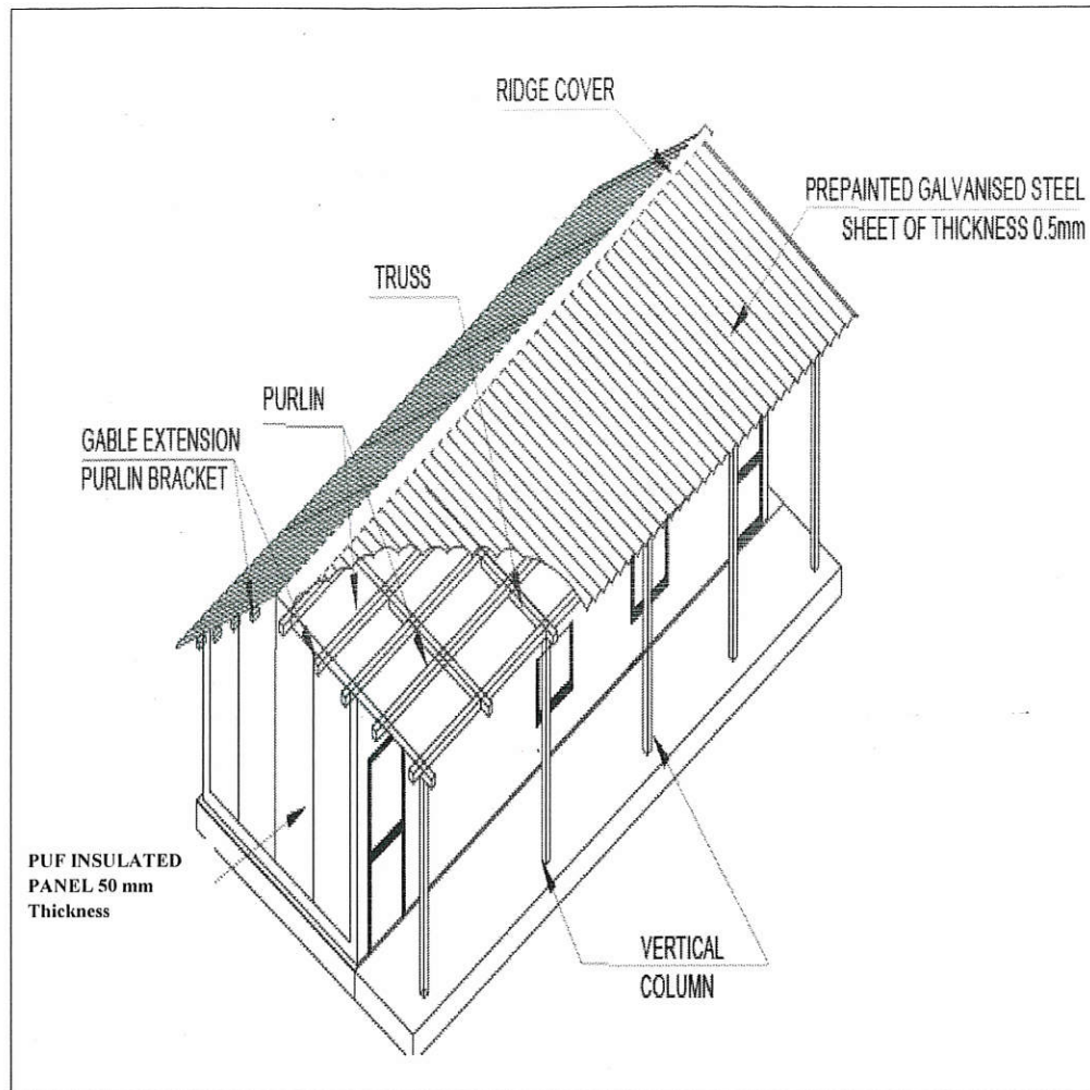
ISOMETERIC VIEW
