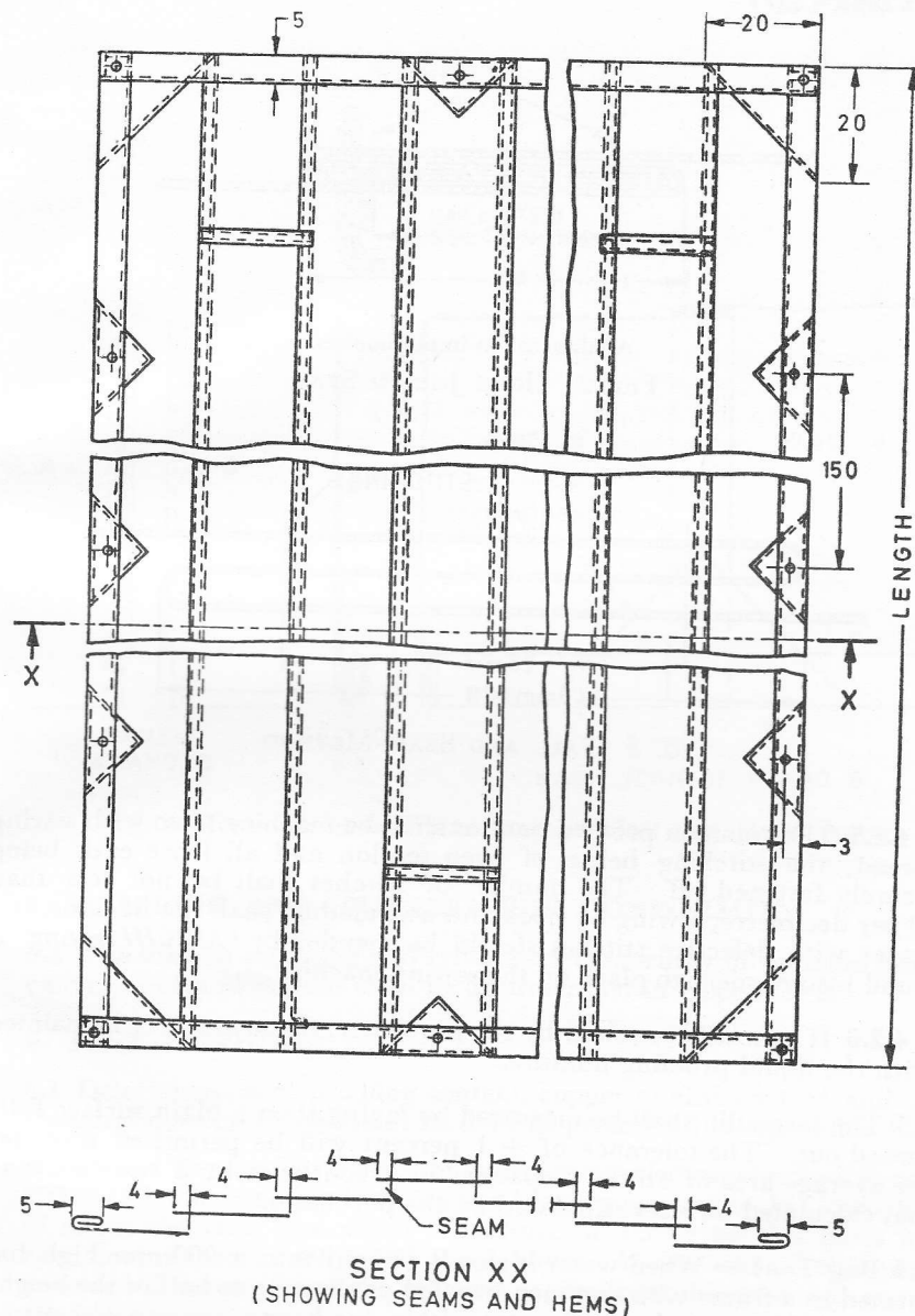
FIG. 1 CONSTRUCTION OF COMMON PROOFED PAULINS ( TARPULINS )
