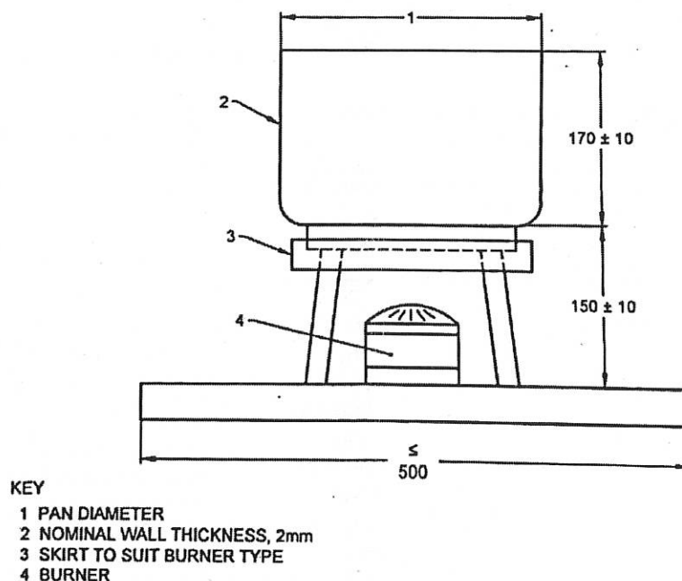
FIG. 3 GENERAL DIMENSIONS FOR CLASS F TEST APPARATUS — TYPE A APPARATUS FOR CLASS 5F ONLY
