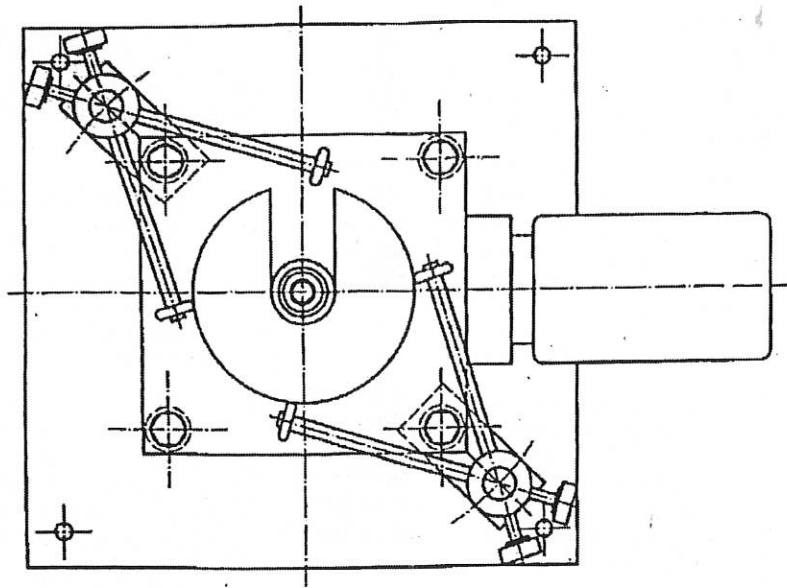
1B View from Above
